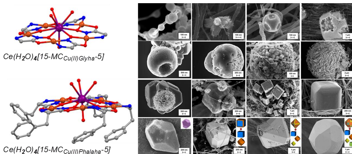
Figure 1. Molecular structures of glycinehydroximate and phenylalaninehydroximate Cu(II)-Ce(III) complexes (left) and SEM images of cerium and copper oxide nanostructures grown hydrothermally from these complexes as single-source precursors (right)
