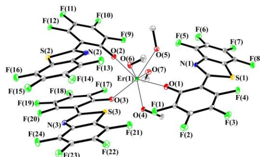
Figure 1. Molecular structure of \text{Er}(\text{SON}^{\text{F}})_3(\text{OCH}_3)_4
