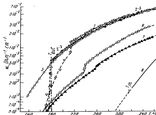
Figure 1. Temperature dependence of specific conductivity of \text{ZnCl}_2\text{--PCl}_5 molten mixtures (1-7) and \text{ZnCl}_2 (8): 1 - 47; 2 - 31; 3 - 30; 4 - 26; 5 - 23; 6 -12; 7 - 6 mol.% of \text{PCl}_5
