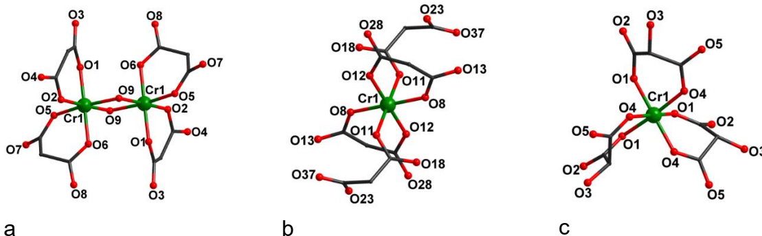
Figure 1. Different types of Cr III -malonate units: dinuclear unit of 1 (a), mononuclear bis-chelate unit of 3 (b, CH 3 groups of Me 2 mal are omitted) and tris-chelate unit of 4 (c) (H atoms are omitted)
