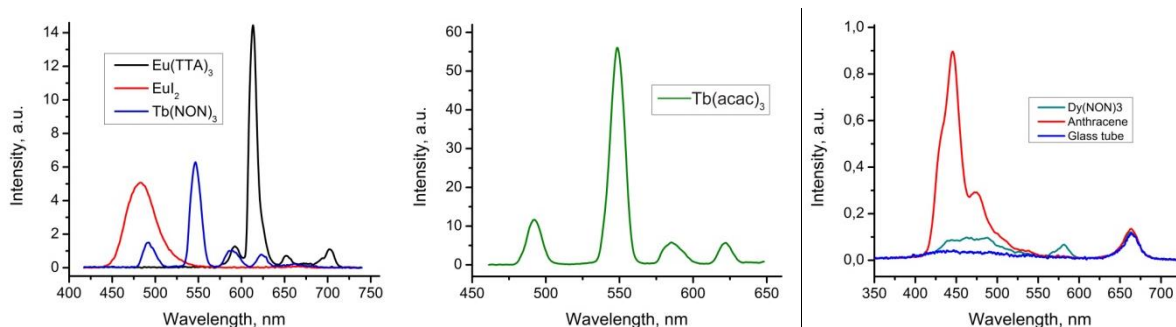
Figure 1. Radio luminescence spectra of organometallic complexes of lanthanides and anthracene
