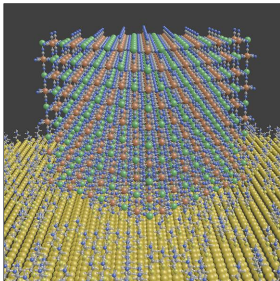
Figure 1. Schematic representation of a Prussian blue analogue nanoparticle on a cysteamine-functionalized gold surface
