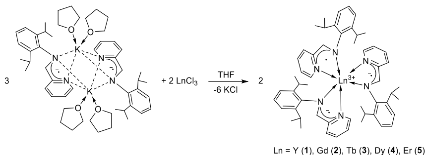
Scheme 1. Synthesis of \text{Ln}^{3+} complexes 1–5 coordinated by radical-anionic iminopyridine ligands
