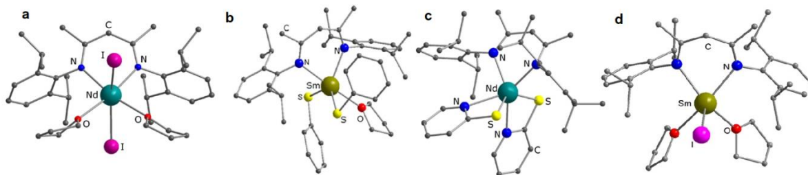
Figure 1. Examples of [Ln(nacnac)I 2 (thf) 2 ] (a), [Ln(nacnac)(SPh) 2 (thf)] (b) and [Ln(nacnac)(SPy) 2 ] (c) complexes; [Sm(nacnac)I(thf) 2 ] (d)
