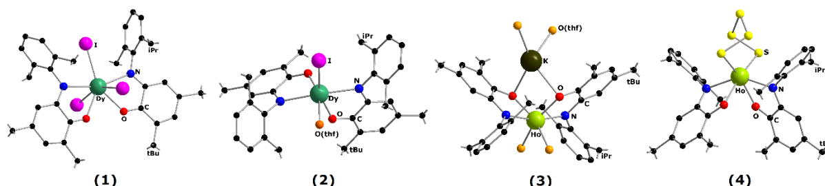
Figure 1. Crystal structures of complexes: [DyI 3 (dipp-IQ) 2 ] (1), [DyI(dipp-ISQ) 2 (thf)] (2), [K(thf) 2 ][Ho(dipp-AP) 2 (thf) 2 ] (3), [K(18-crown-6)(thf) 2 ][HoS 5 (dipp-ISQ) 2 (thf) 2 ] (4)
