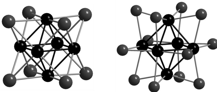
Figure 1. Octahedral cluster cores: \{M_6I_8\} (left), \{M_6I_{12}\} (right)
