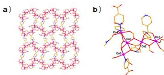
Figure 1. Representations of the a) 3D porous structure and b) Co 5 repeating unit of Co 5 -INA.
