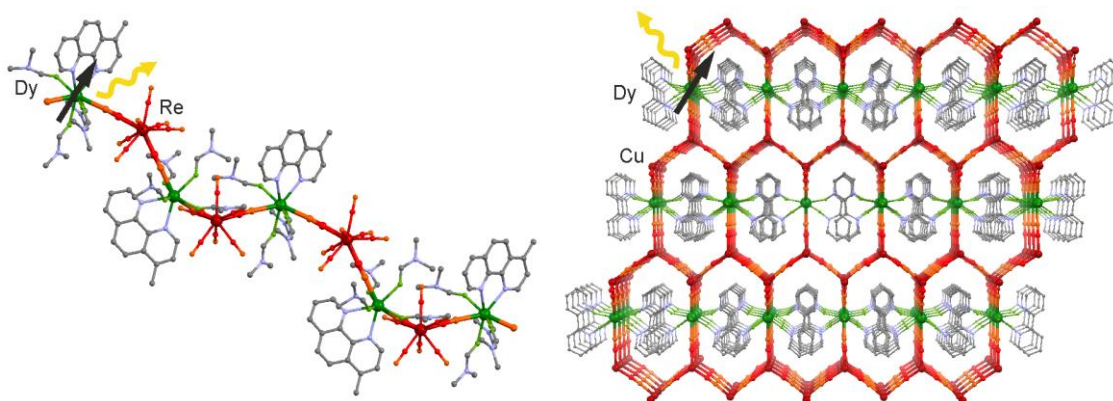
Figure 1. Bimetallic \text{Dy}^{\text{III}}[\text{M}(\text{CN})_x]^{n-} coordination systems incorporating luminescent Dy(III) SMMs
