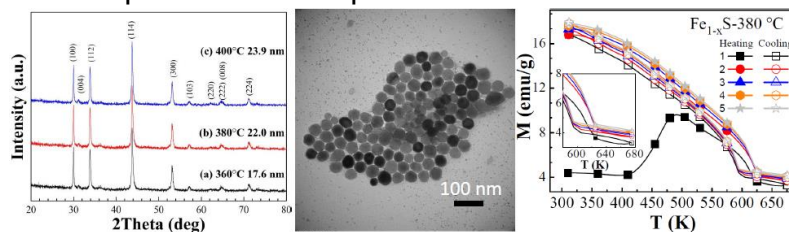
Figure 1. (a) XRD patterns of \text{Fe}_{1-x}\text{S}@\text{C} NPs prepared at different temperatures; (b) TEM image and (c) Temperature-dependent magnetization M_{H=1.5T} , obtained from hysteresis loops of \text{Fe}_{1-x}\text{S}@\text{C} NPs synthesized at T_R = 380 °C.
