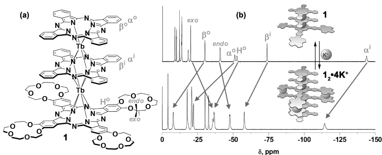
Figure 1. (a) Heteroleptic complex 1, (b) ^1\text{H} -NMR spectra for complex 1 and supramolecular dimer 1_2 \cdot 4\text{K}^+ in \text{CDCl}_3 + 20\text{vol.}\% \text{CD}_3\text{OD} .
