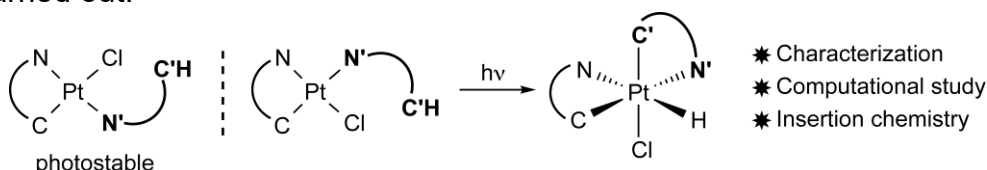
Figure 1. C ^ N: Cyclometalated 2-arylpyridine.
