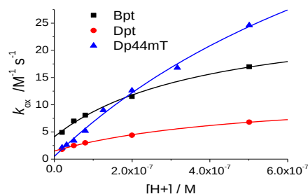
Figure 1. [H + ]-dependence of the second order rate constants ( k_{ox} ) for the oxidation of the Fe II bis -thiosemicarbazone complexes (left) studied at 25 °C
