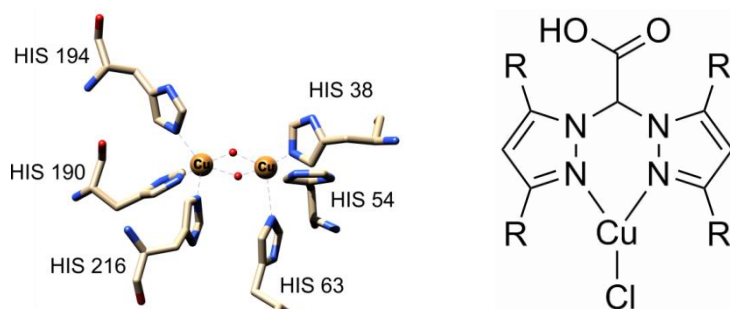
Figure 1. A) Tyrosinase as an example of dinuclear type 3 copper enzymes. (PDB 3AWV) B) Cuprous complexes bearing bis(3,5-disubstituted pyrazol-1-yl)acetic acids ( \text{R} = \text{'Bu} ( 1 ), \text{Ph} ( 2 ))
