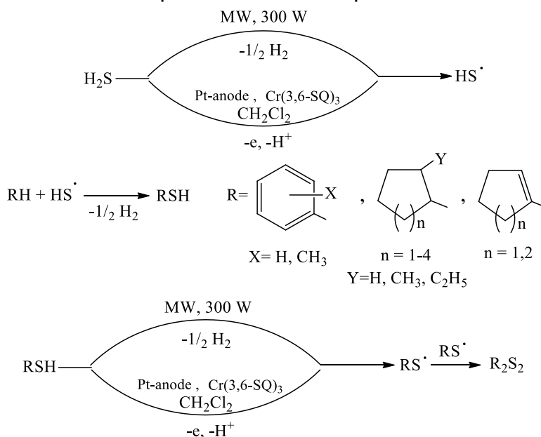
Figure 1. Scheme of the radical reaction mechanism of organic compounds thiolation under different conditions of \text{H}_2\text{S} activation
