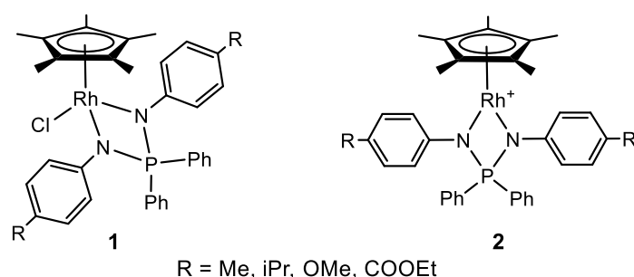
Figure 1. Half-sandwich 18 \bar{e} and 16 \bar{e} rhodium iminophosphonamides
