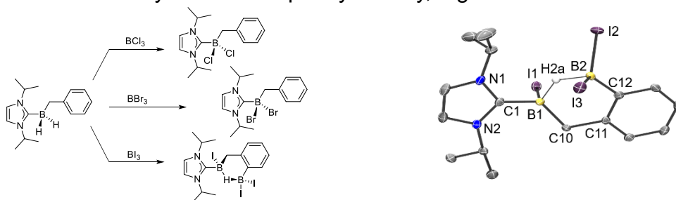
Figure 2. \text{IiPr} -benzylborane and its reactivity towards borontrihalides (left), crystal structure of bisborylated product (right)
