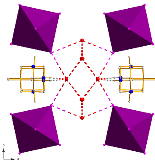
Figure 1. View of the crystal structure of (\text{C}_{10}\text{N}_2\text{H}_{19})_2(\text{H}_3\text{O})\text{BiI}_6 \cdot 5\text{H}_2\text{O}
