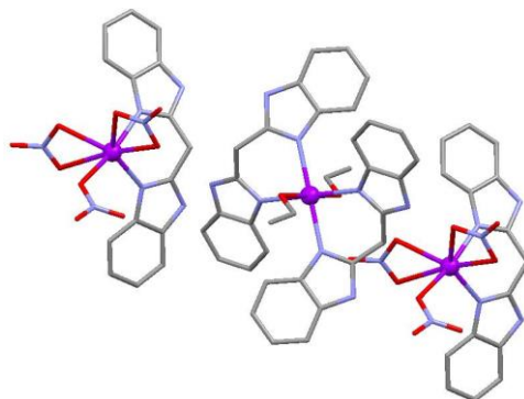
Figure 1. Structure of [Cd(L^1)_2(EtOH)_2][Cd(L^1)(NO_3)_3] \cdot 2 \cdot 6EtOH
