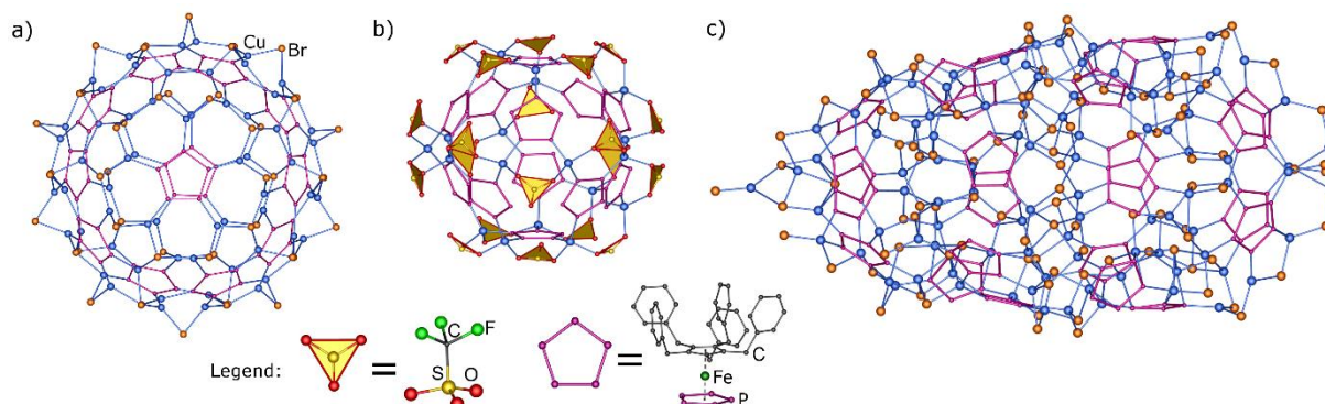
Figure 1. Molecular structure of the cores of superspheres a) [(Cp^{Bn}FeP_5)_{12}Cu_{70}Br_{83}] with I-C 140 topology of the outer shell, b) D 2 isomer of [(Cp^{Bn}FeP_5)_{12}(CuOTf)_{20}] and c) rugby-ball [(Cp^{Bn}FeP_5)_{24}(CuBr)_{96}] .
