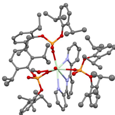
Figure 1. Structure of [(\text{iPr}_2\text{C}_6\text{H}_3\text{O})_2\text{PO}_2]_3\text{Nd(terpy)(MeOH)(H}_2\text{O)}
