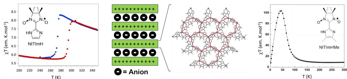
Figure 1: Temperature dependence of \chi T for \{[\text{Mn}_2(\text{NITIm})_3]\text{ClO}_4\}_n and \{[\text{Mn}_2(\text{NITImMe})_3]\text{ClO}_4\}_n
