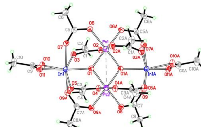
Fig. 3. Molecular structure of tetranuclear complex Pt 2 (O) 2 In 2 (OOCMe) 10
