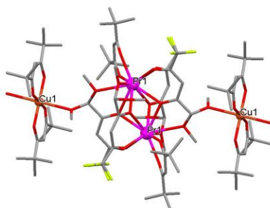
Figure 1. A fragment of [(\text{PrL}_2(\text{thd}))_2\text{Cu}(\text{thd})_2] coordination polymer. L= trifluoro-5,5-dimethoxypentane-2,4-dionate, thd= 2,2,6,6-tetramethylheptane-3,5-dionate
