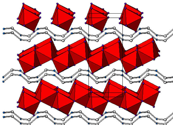
Figure 1. View of the crystal structure of \text{KBiI}_4 \cdot \text{H}_2\text{O} 3
