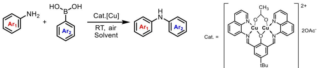
2. The Chan-Evans-Lam reaction
