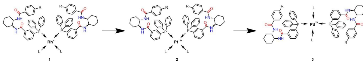
Figure 1. Catalytically active Rh complexes 1 which are modeled by Pt complexes 2 and the Pd complexes 3 currently under investigation
