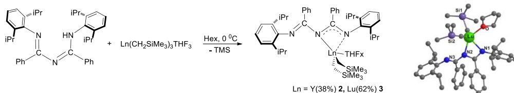
Scheme 1. The synthesis of bis(alkyl) rare-earth complexes 2 and 3
