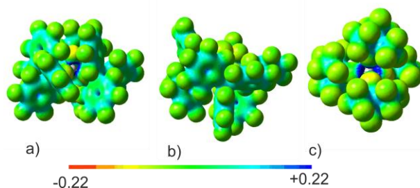
Figure 1. Projection of the calculated electrostatic potential on the 0.025 \text{ e}^- \text{ Bohr}^{-3} isodensity surface.
