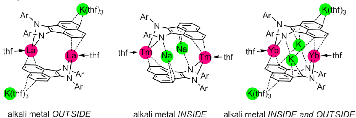
Figure 1. Lanthanide complexes with tetraanion of dpp-bian
