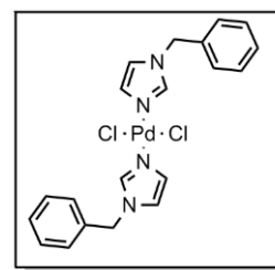
Figure 4. The imidazole complex
