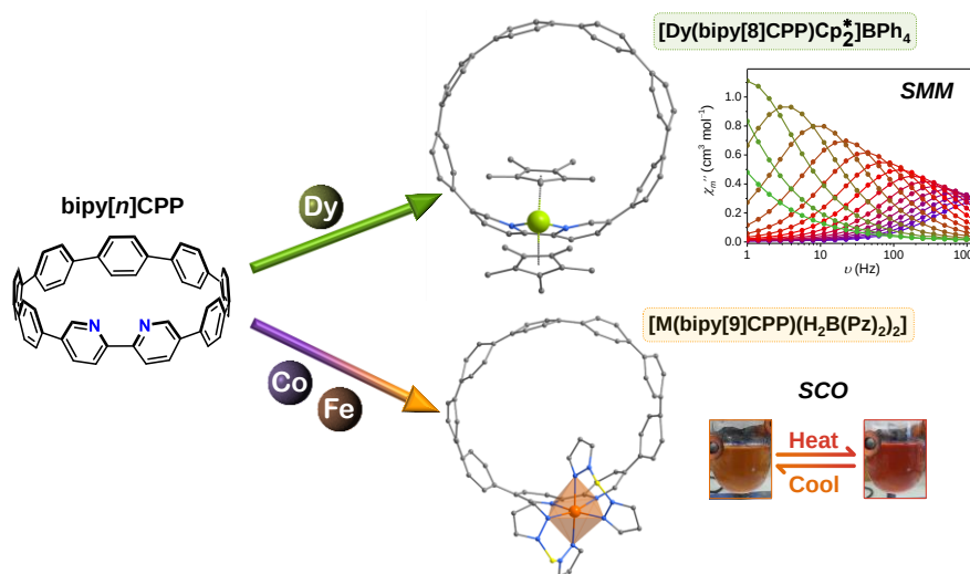
Figure 1. Design and physical properties of 3d/4f-nanohoop systems
