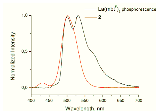
Figure 2. PL spectra of La(mbt F ) 3 and 2 in solid state
