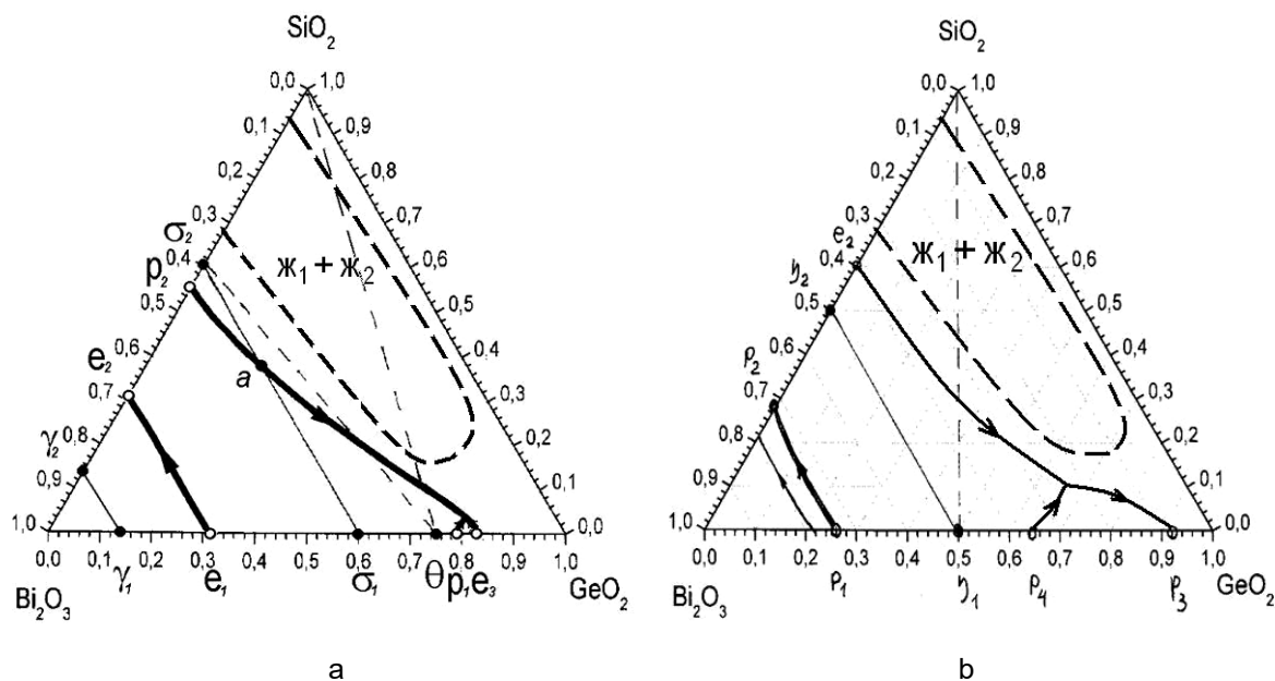
Figure. Projections of the liquidus surface in the system \text{Bi}_2\text{O}_3\text{-SiO}_2\text{-GeO}_2 in stable (a) and metastable (b) equilibria
