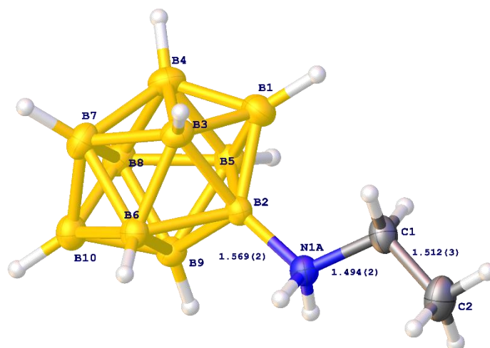
Figure 1. Structure of the [B 10 H 9 NH 2 Et] − anion
