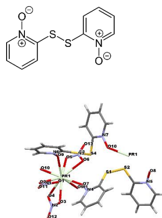
Figure 2. 2,2'-dithiobis (pyridine-Noxide)
