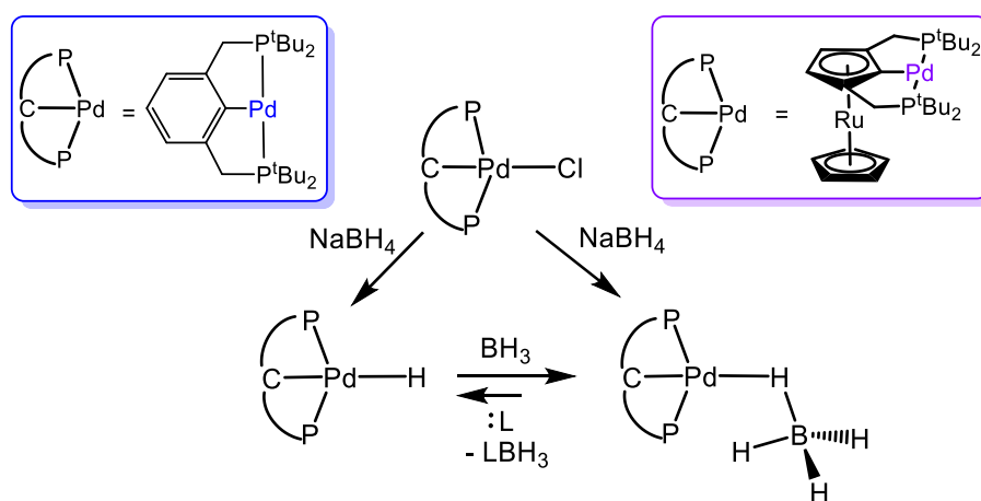
Figure 1. General scheme of formation of pincer (pincer)PdX complexes
