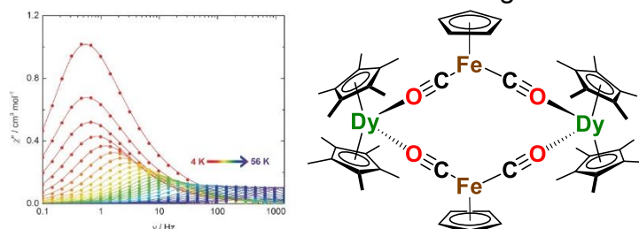
Figure 1: A 4f/3d carbonyl bridged dimer, DyFp , demonstrating SMM behaviour
