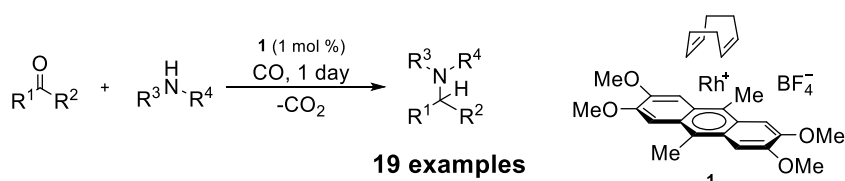
Figure 1. Reductive amination
