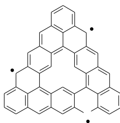
Figure 1. Holed triangulene, S=3/2
