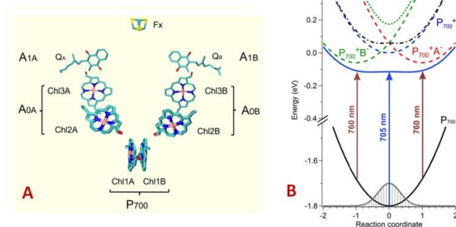
Figure 1. A. Scheme of reaction center in PS I.
