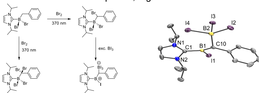
Figure 3. UV induced radical bromination of \text{IiPr-BBr}_2\text{Bn} and subsequent reaction with \text{BI}_3 (left), crystal structure of zwitterionic species (right)
