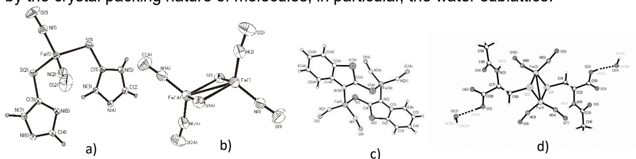
Figure 1. a) mononuclear dinitrosyl DNIC; b) Red Roussin's Salt – DNIC of \mu -S structure type; c) DNIC with 2-mercaptobenzthiazole of \mu -N-C-S type; d) DNIC with acetylcysteine.
