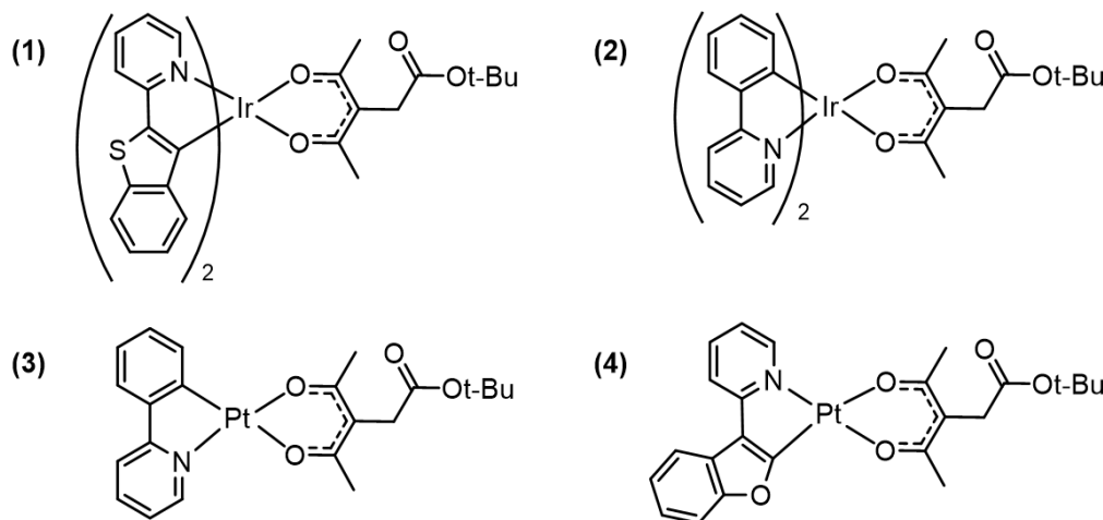
Figure 1. Structures of the complexes 1-4
