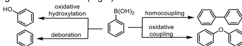
Figure 1. Side reactions in CEL-coupling
