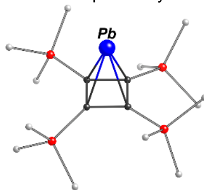
Figure 1. Plumbapyramidane.
