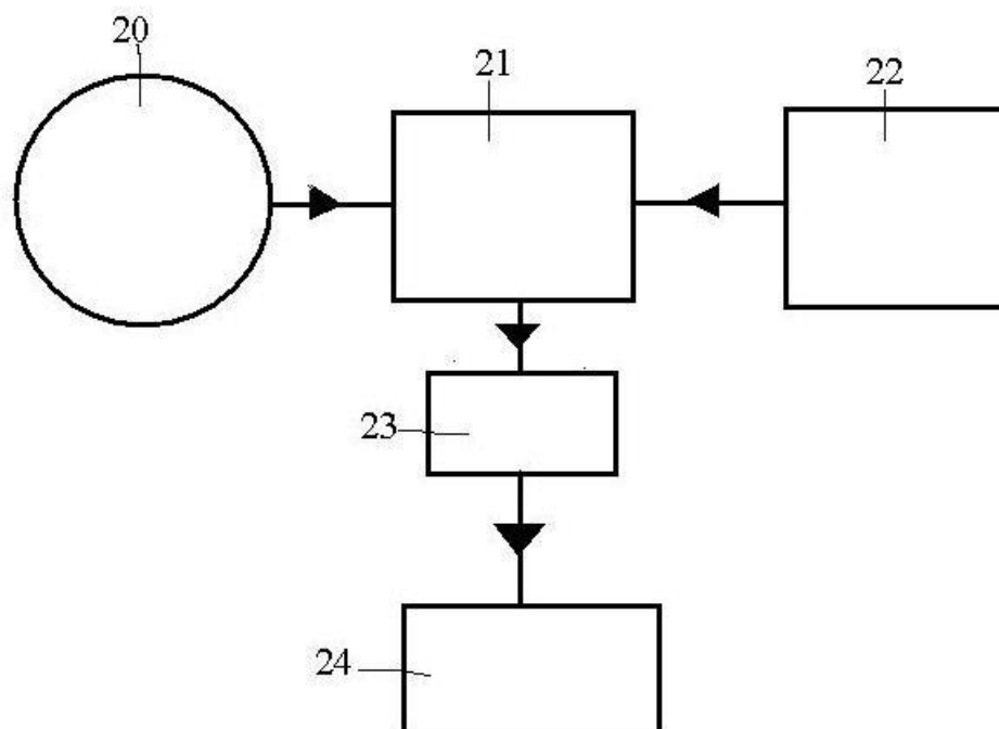
Fig. 2. TF Receiver. 20 - spherical metal sensor; 21 - mixer/multiplier; 22 - source of the video signal of image of the receiver or combined image of the receiver and transmitter; 23 - low-pass filter; 24 - output device.
