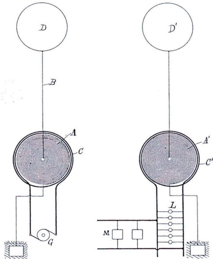
Figure1. Tesla Coils in N.Tesla's patent, No.649.621
