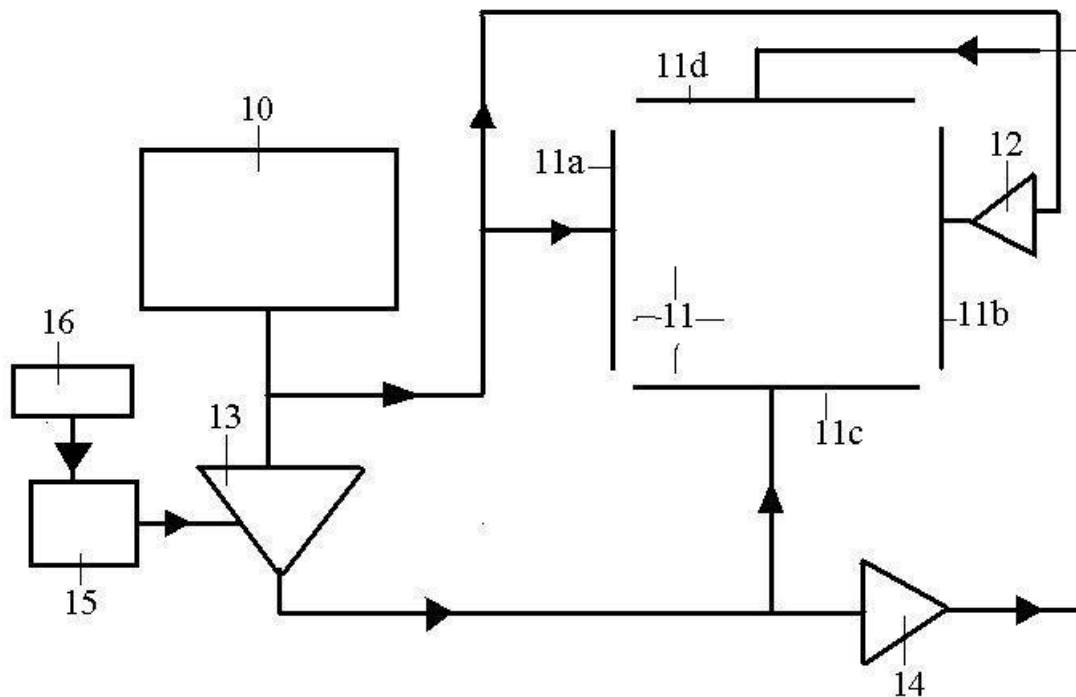
Fig. 1. TF Transmitter. 10 - source of the video signal of image of the receiver or combined image of the receiver and transmitter; 11 - electric quadrupole; 11a,b,c,d plates of the quadrupole 11; 12 - inverter; 13 - differentiator; 14 - another inverter; 15 - modulator; 16 - source of transmitted information.
