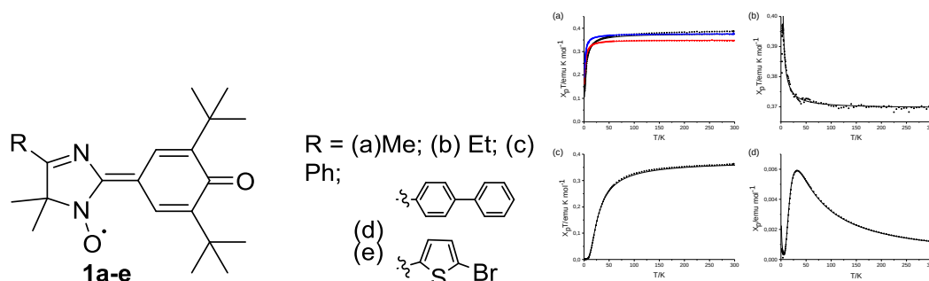
Fig.1. The SQUID magnetometry of the polycrystalline (solid) radicals 1a-e : (a), (b) and (c) \chi_{para}T vs. T plots for (a) 1a (black);, 1b (red); 1d (blue); (b) 1c ; (c) and (d) 1e . The dotted curves denote the experimental values and the solid curves the calculated Curie-Weiss curves in (a),(b) or Bleany-Bowers curve ( J/k_B = -25.6 K + Curie curve in (c) and (d).
