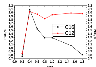
Fig. 2 PCE versus P3HT/IMF-C12 (C16) weight ratio
