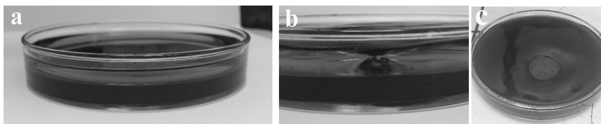
Figure 1(a, b, c) – Stages of formation reduced graphene oxide film: (a) heating of the oil layer; (b) formation at the interface of oil and water dispersion of reduced graphene oxide film; (c) transition reduced graphene oxide film through oil layer
