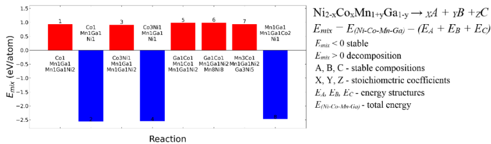
Fig. 1. Formation energy and decomposition reaction for the composition Ni_{31}Co_1Mn_{16}Ga_{16}
