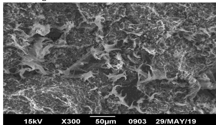
Fig. 1. Microstructure of a 15% LDPE/55% C/30%LSMO cleaved sample.
