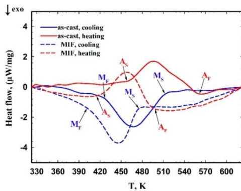
Fig. 1. Comparison of DSC curves of the alloy in the as-cast state and after forging.
