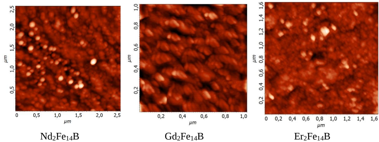
Fig. 2. Atomic-force microscopy microstructures of R_2Fe_{14}B ( R = Nd, Gd, Er ) quenched with 20 m/s drum rotation speed.
