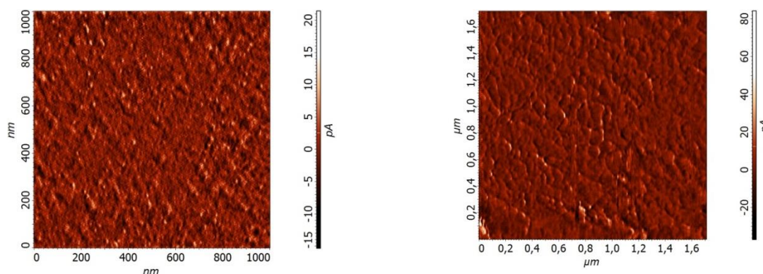
Fig. 1. Microstructure of Y_2Fe_{14}B quenched with 20 m/s (left) and 30 m/s (right) drum rotation speed obtained using atomic-force microscopy.
