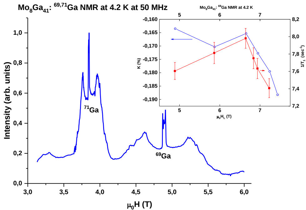
Fig. 1. \text{Mo}_8\text{Ga}_{41} field-sweep NMR spectrum at 50 MHz and 4.2 K. Inset: ^{69}\text{Ga} Knight shift (left) and spin-lattice relaxation rate (right) as a function of magnetic field.
