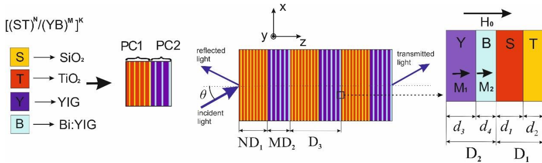
Fig. 1. Schematic of the 1D three-periodic magnetic crystal [(\text{SiO}_2/\text{TiO}_2)^N/(\text{YIG}/\text{Bi:YIG})^M]^K .
