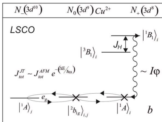
Fig.4 Jahn-Teller interaction \sim I\varphi \cdot [\delta(\theta - 45^\circ) + \delta(\theta - 135^\circ)] in N_+ sector of configuration space for D stripes with (A_g + B_{1g}) \otimes (a_{1g} + b_{1g}) instability.
