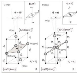
Fig. 1 Tilting of \text{CuO}_6 octahedra in U(b) and D(a) stripes between rock salt layers LaO.
