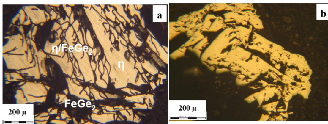
Fig. 2. Optical micrographs of the high-pressure-synthesized FeGe sample after (a) and before (b) DSC heating.
