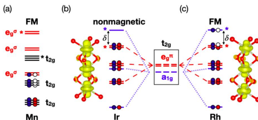
Figure 1: (a) Level diagram (with both t_{2g} and e_g ) for Mn trimer (localized electrons) and (b), (c) scheme of t_{2g} energy levels (no e_g ) for MO model and charge densities of the band above/at the Fermi level for (b) Ir and (c)
