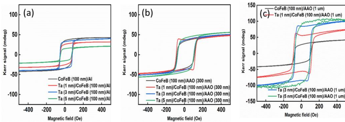
Fig. 1 Control of the MOKE rotation of Ta ( x ) /CoFeB/substrate thin films by the Ta layer thickness for different substrates: (a) Al plate; (b) AAO template with pore diameter of 100 nm and depth of 300 nm; (c) AAO template with pore diameter of 100 nm and depth of 1000 nm.
