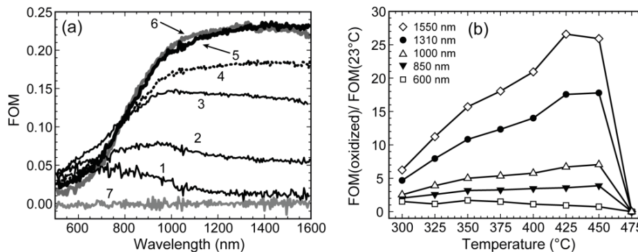
(a) Changes in FOM = \theta_F \sqrt{T} for the nanofilms: initial permalloy nanofilm (curve 1) and oxidized ones during annealing for one hour at the series of temperatures (curves 2-7 correspond to 300, 350, 400, 425, 450 and 475°C, respectively). (b) Normalized FOM for selected wavelengths versus the oxidation temperature.
