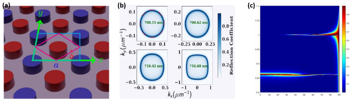
Fig. 1 (a) 2-d square lattice with dimension of alternating dielectric discs in a row changed. (b) RCWA calculated reflection coefficient showing circular symmetry for quasis-BIC region and broken circular symmetry for leaky modes. (c) Numerical simulations showing the Berreman and epsilon near zero modes.
