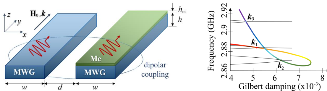
Fig. 1. The investigated magnonic system, where backward volume waves are excited (left); exceptional point dependence on wave number, k_1 = 1 rad/ \mu\text{m} , k_2 = 10 rad/ \mu\text{m} , k_3 = 30 rad/ \mu\text{m} (right).
