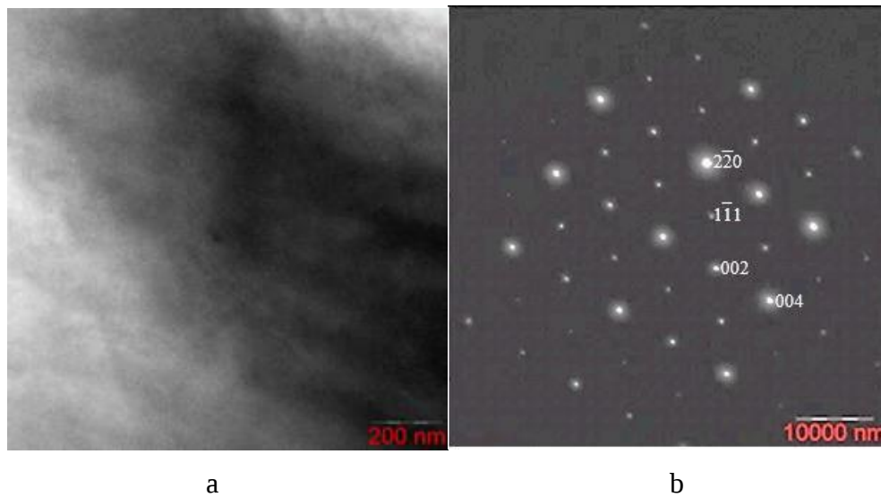
Fig. 2 Microstructure of the austenitic phase of the \text{Ni}_{46}\text{Mn}_{41}\text{In}_{13} alloy: a - bright field image; b - electron diffraction pattern, zone axis [110]_{\text{L21}} .
