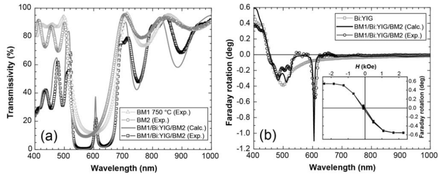
(a) Transmission spectra of BM 1 annealed at 750 °C for 45 minutes, as-deposited BM 2 and fabricated MPC ( (\text{ZrO}_2/\text{SiO}_2)^7/\text{Bi:YIG}/(\text{ZrO}_2/\text{SiO}_2)^7 ); the calculated spectrum is given by a solid line. (b) Angle of Faraday rotation of the single Bi:YIG film (squares) and MPC; measured and calculated dependencies for MPC are shown as circles and a solid line, respectively. Inset illustrates a hysteresis curve of Faraday rotation for MPC.
