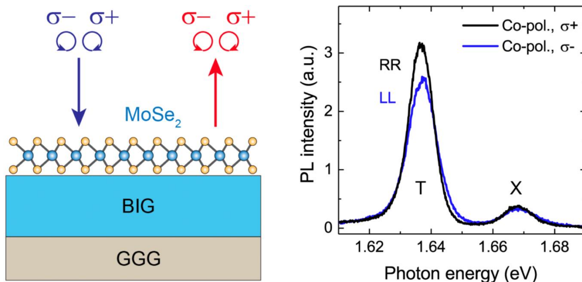
Fig. 1. Left is the principle scheme of the sample, consisting of monolayer \text{MoSe}_2 transferred onto thin film of bismuth iron garnet (BIG) on gadolinium gallium garnet (GGG) substrate, and types of different excitation/detection with circular polarization. Right – is the typical photoluminescence spectra from the \text{MoSe}_2 monolayer positioned on the magnetic film. T marks the area of the trion peak, X is the area of the neutral exciton.
