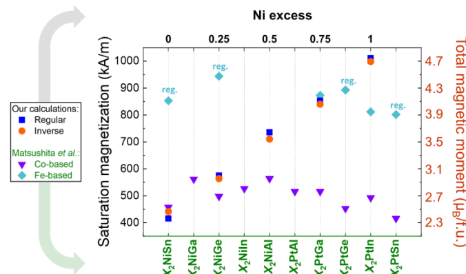
Fig. 1. Saturation magnetization and total magnetic moments for \text{Co}_2\text{Ni}_{1+x}\text{Sn}_{1-x} ( x = 0, 0.25, 0.5, 0.75, 1 ) in comparison with other Co- and Fe-based Heusler systems [3].
