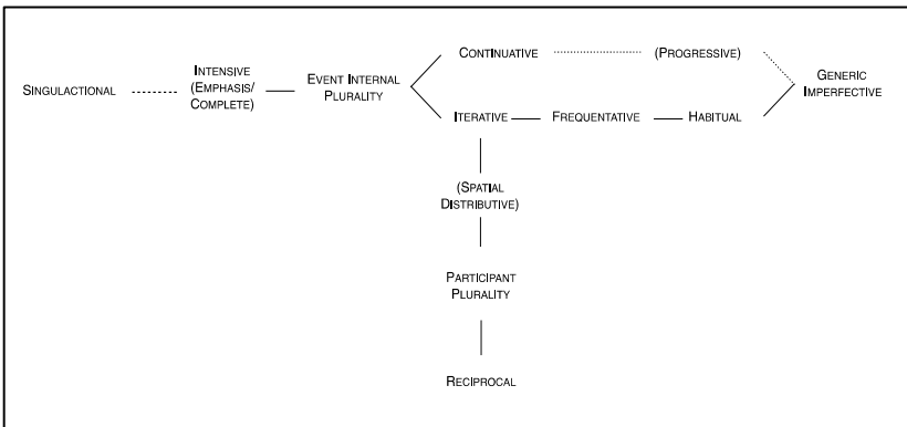
Figure 1. Semantic map
